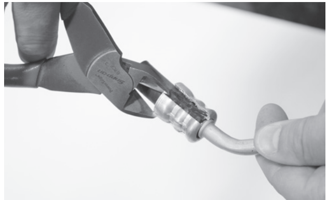
Figure 26: Modifying power steering return line
