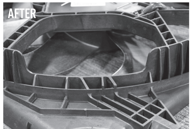
Figure 34: Modify fan shroud
